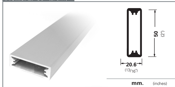
Profile: EF-50 (EPOXY)
